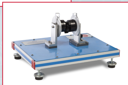
MGI Gyroscope
