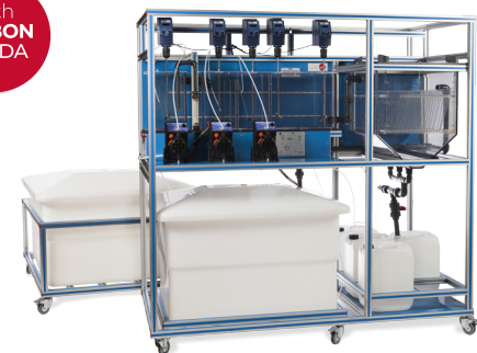
SPFC Computer Controlled Sedimentation, Precipitation and Flocculation Unit
